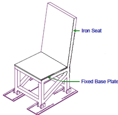
Figure C-6 – ATD Test Seat Setup
