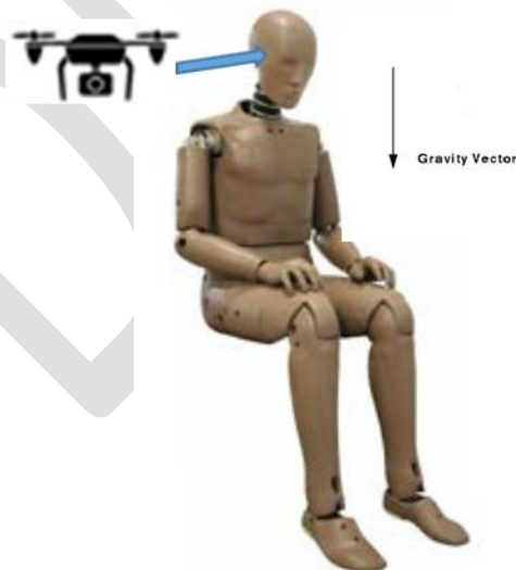
Figure C-4 – Head Side Impact Test Configuration
